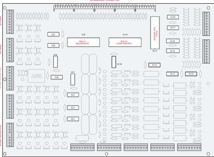
2 DRIVER BOARD
