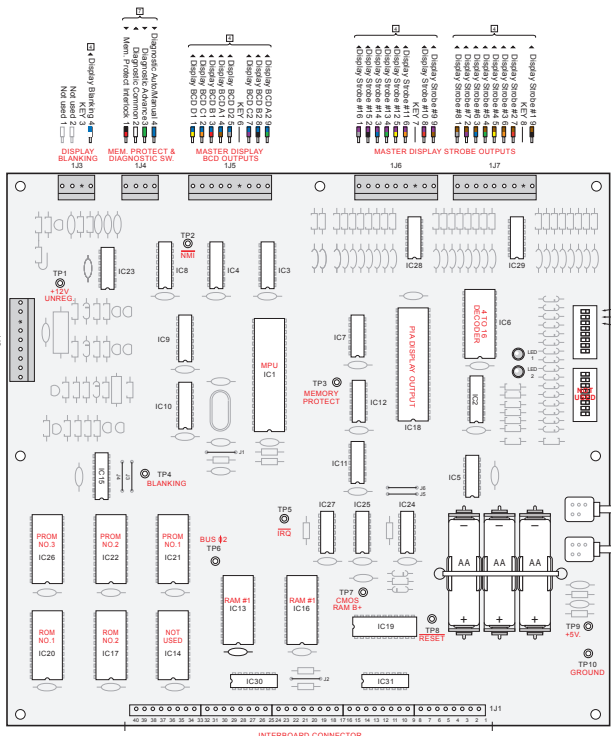
1 CPU BOARD
